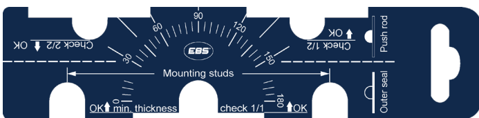
Brake Chamber Alignment Tool REF: EBS.BCAT
